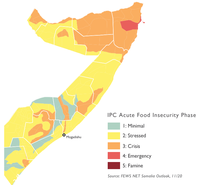
Projected Acute Food Insecurity, February Through May 2021
