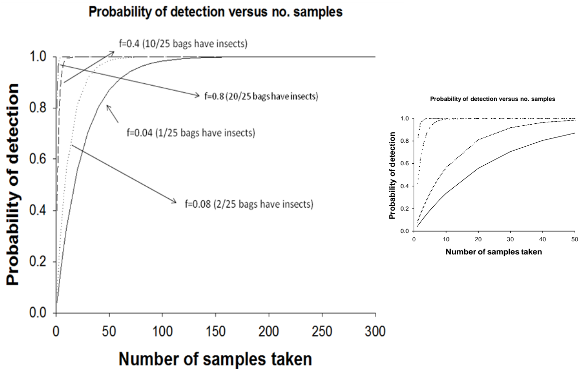
Figure 1. Relationship between Probability of Detection, Number of Samples, and Frequency of Infestation. The Inset Graph Shows the Same Four Lines Over 0 to 50 Samples.
